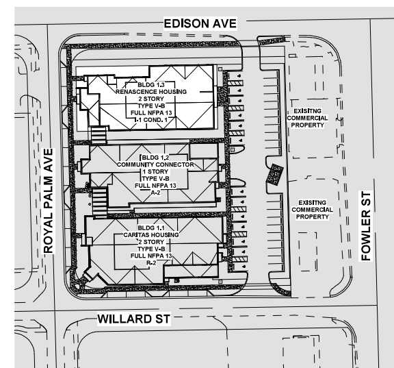
3 ARCHITECTURAL SITE PLAN PARTIAL 1" = 40'-0"
